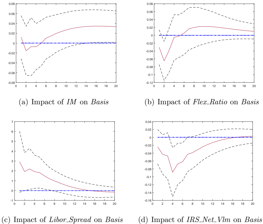
Figure 2: Impulse response functions obtained from estimating model (13). The CME-LCH basis defined in equation (9). IM is the total initial margin posted by swap dealers on LCH, Flex\_Ratio is the fraction of volume across all SwapClear products that dealers transact with non-dealer banks, Libor\_Spread is the difference between the three-month USD Libor rate and the overnight federal funds rate and IRS\_Net\_Vlm is the client net (i.e. buy minus sell) volume in USD interest rate swap contracts cleared in LCH. The dotted lines show the 95% confidence intervals of the estimated impulse responses.
